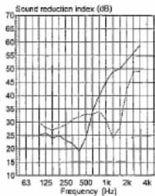
— Sandwich panel with a mineral wool core density 45 kg/m 3 , R_w = 33 dB - - - Sandwich panel with a mineral wool core density 150 kg/m 3 , R_w = 31 dB
