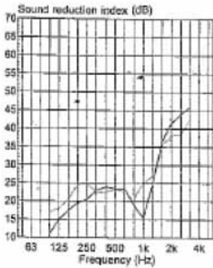
(b) - - - Profilled sandwich panel with a PUR foam core with thickness 65 mm and weight 14 kg/m 2 , R_w = 27 dB — Sandwich panel with a PUR foam core thickness 80 mm and weight 14 kg/m 2 , R_w = 25 dB
